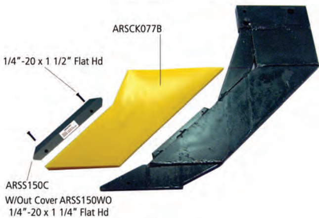
KMC Steel Shank 16-080-077 Width = 1" KMC did not change part# when brace was added.
