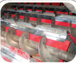
16 Case Auger Bed Liner
