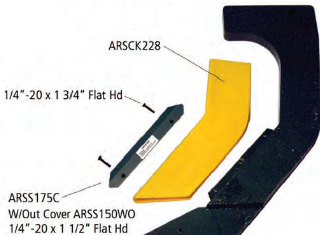
KMC Steel Shank 16-080-228 Width = 1 1/4"
